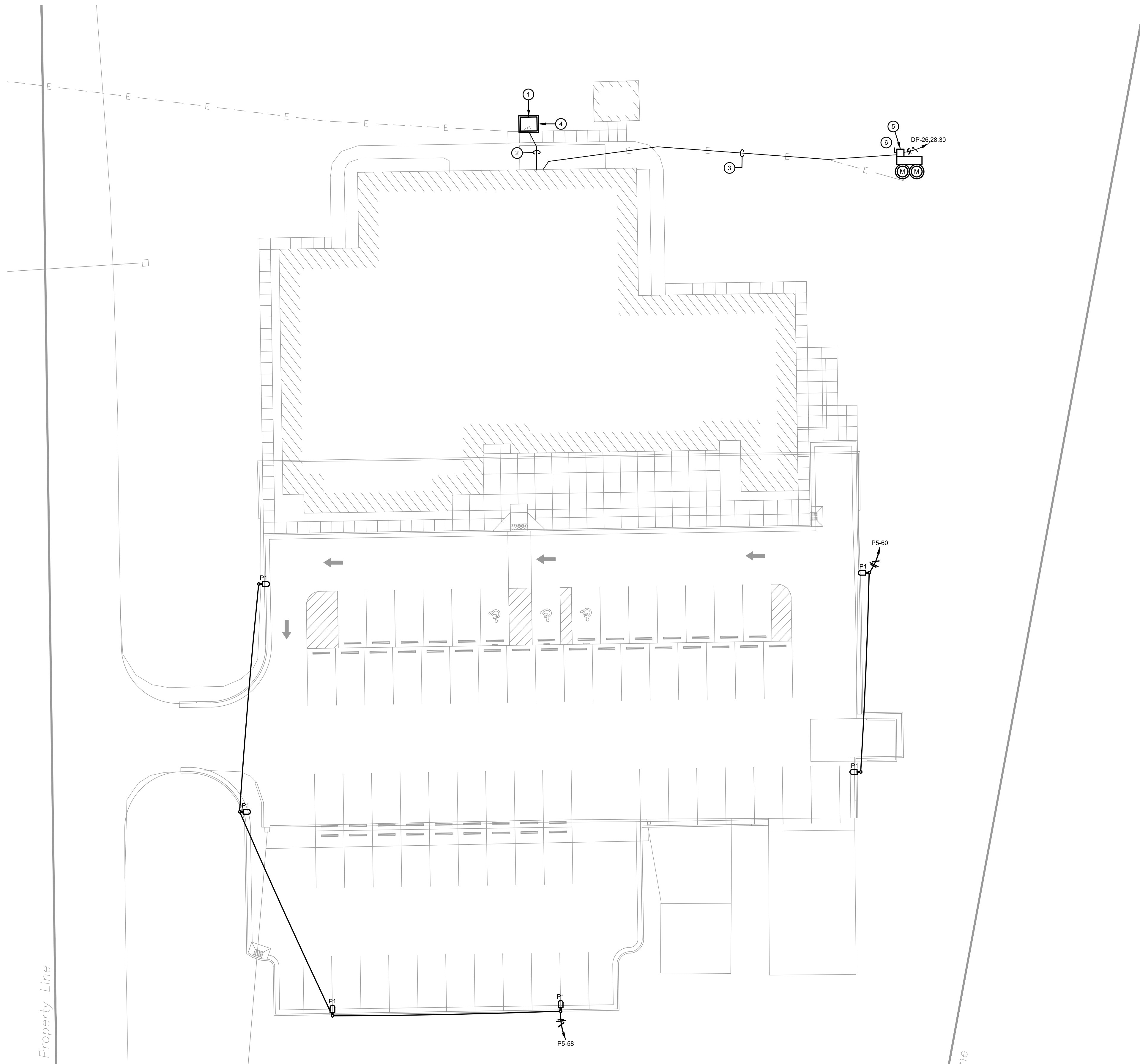
1 ELECTRICAL SITE PLAN E-001 SCALE: 1" = 20'-0"
